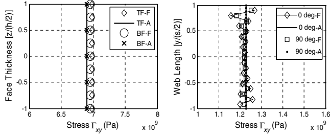
Fig. 16 Shear stresses in the top face, bottom face, and web for a unit-cell strain of \gamma_{xy^M}^M = 1 .
