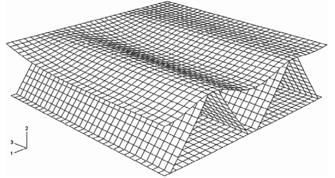
Fig. 23 Exaggerated deformed mesh (deformation scale factor = 2).
