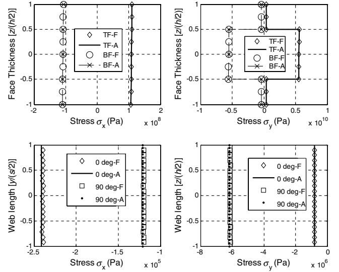
Fig. 18 Stresses in the x and y direction in the top face, bottom face, and web for a unit-cell strain of \kappa_{y^M}^M = 1 .
