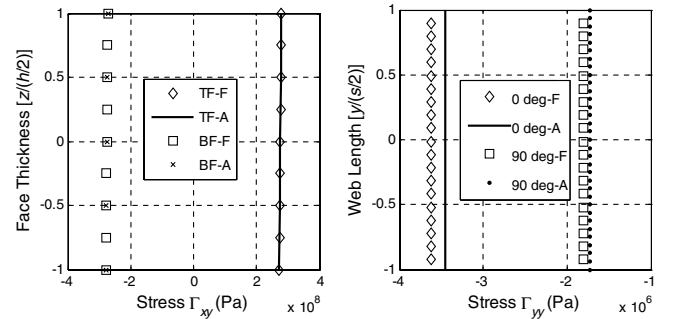
Fig. 19 Shear stresses in the top face, bottom face, and web for a unit-cell strain of \kappa_{xy^M}^M = 1 .
