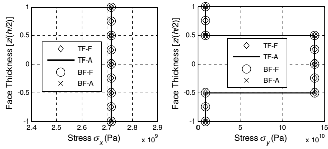
Fig. 15 Stresses in the x and y direction in the top face and bottom face for a unit-cell strain of \epsilon_{y^M}^M = 1 .
